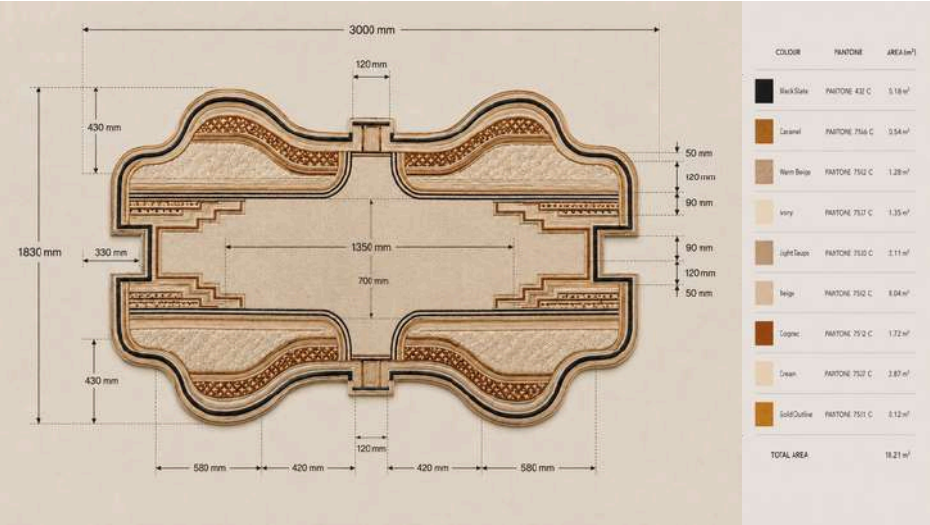
PLAN VIEW
